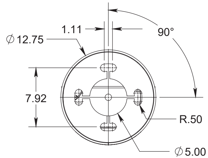
BASE PLATE DETAIL SCALE 1:8
