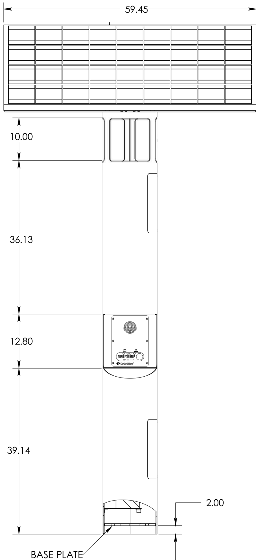
FRONT VIEW
