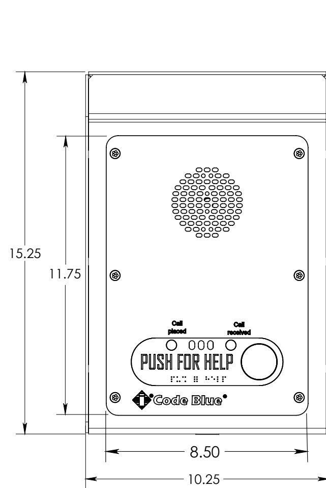
FRONT VIEW
