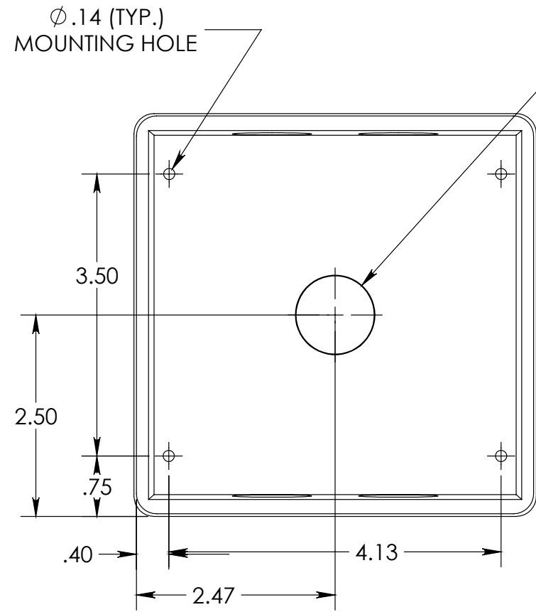
BACK VIEW
