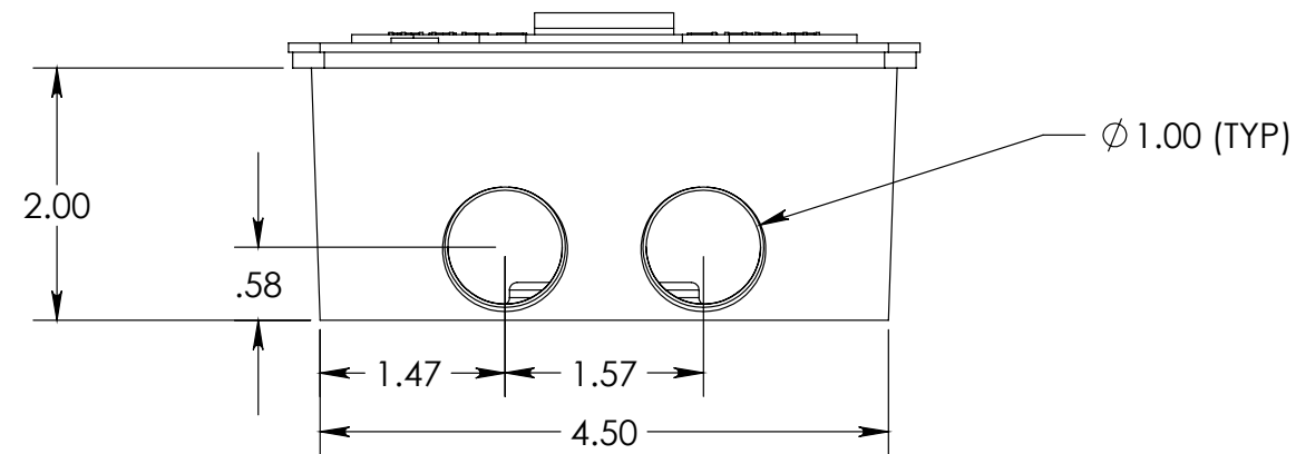
TOP/BOTTOM VIEW
