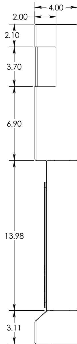
SIDE VIEW
