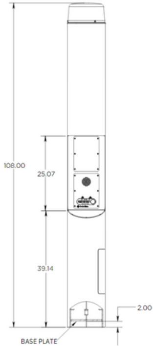
CB 1-e w/ Dual Faceplates
