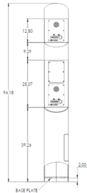
CB 9-t w/ Single & Dual Faceplates
