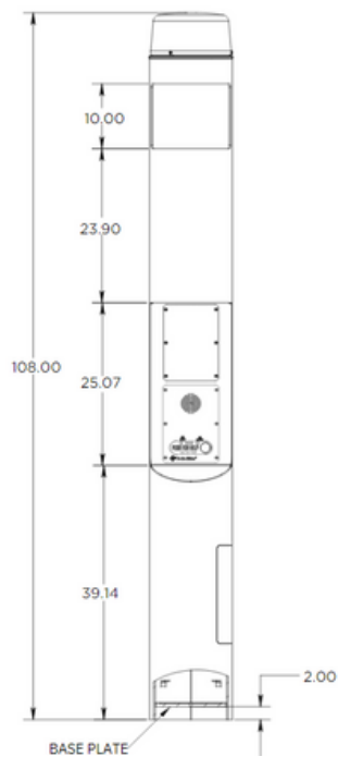
CB 1-s w/ Dual Faceplates
