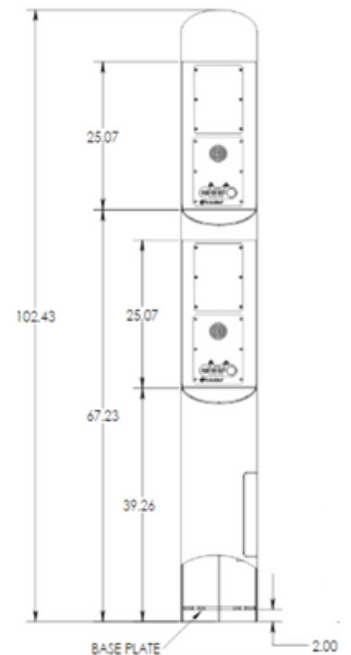
CB 9-t w/ 2x Dual Faceplates
