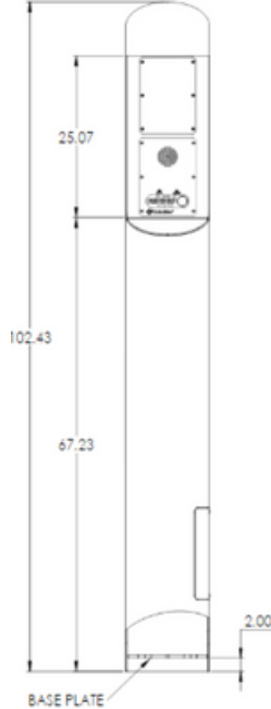
CB 9-t w/ Dual Faceplates
