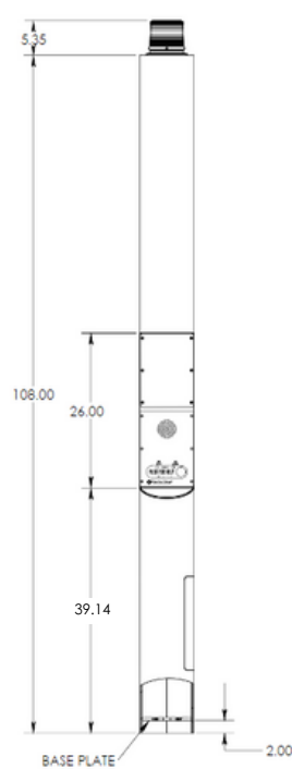
CB 5-s w/ Dual Faceplates
