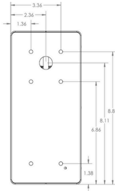
BACK VIEW
